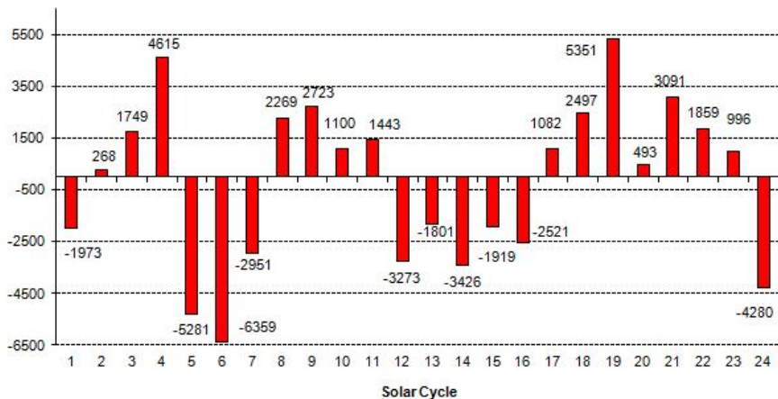
Accumulated monthly Sunspot Anomaly until 116 month after cycle start
