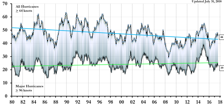
Global Major Hurricane Frequency – 12 month running sums
