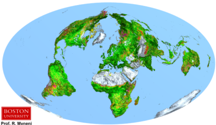
Change in Leaf Area (% 1982 to 2015)
