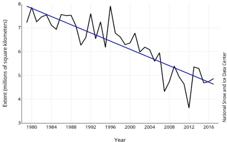
Average Monthly Arctic Sea Ice Extent September 1979 - 2017
