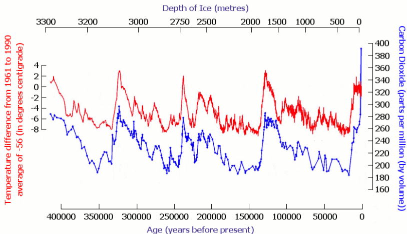
The Vostok (Antarctica) Ice Core Record. Carbon Dioxide versus Temperature for the last 420,000 years.
